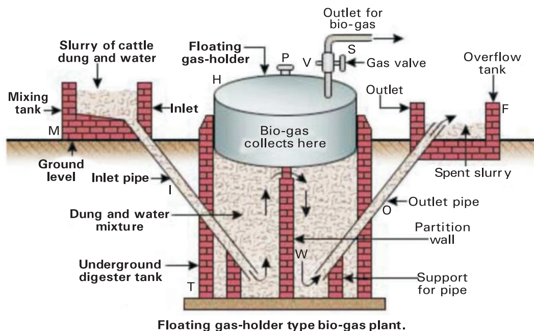
Figure 11.17 Biogas Plant
