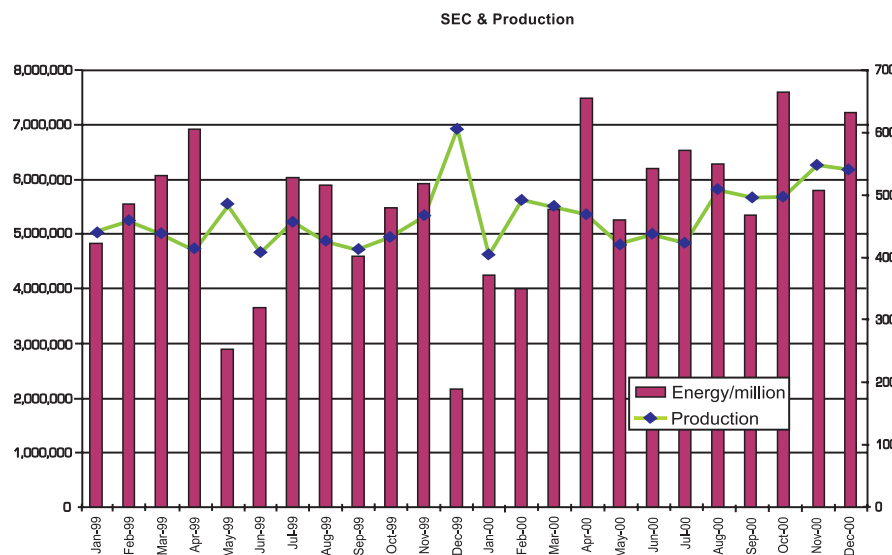
Figure 9.8 SEC with Production
