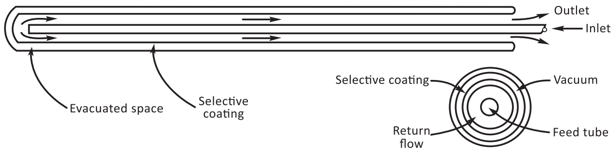
Figure 11.4 Cut view of Evacuated Tube Collector
