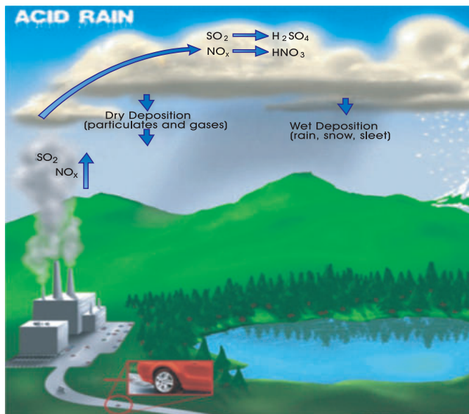
Figure 10.2 Acid Rain Formation
