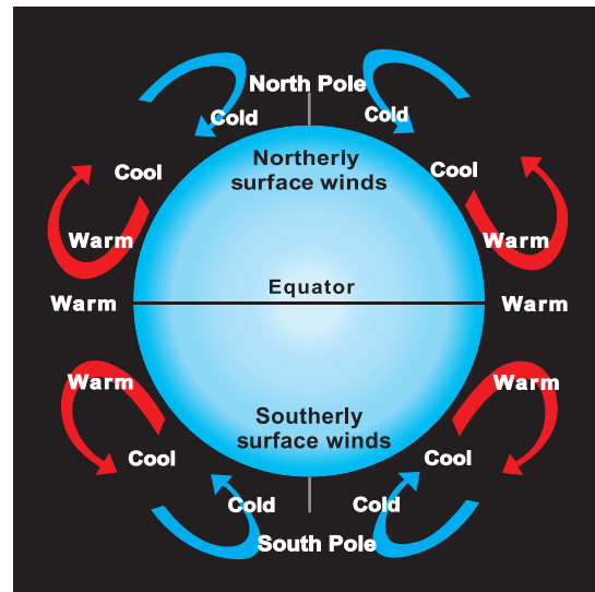
Figure 11.11 Global Wind Flow
