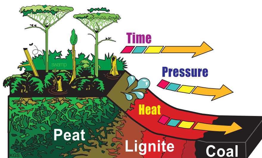
Figure 1.3 Formation of Coal
