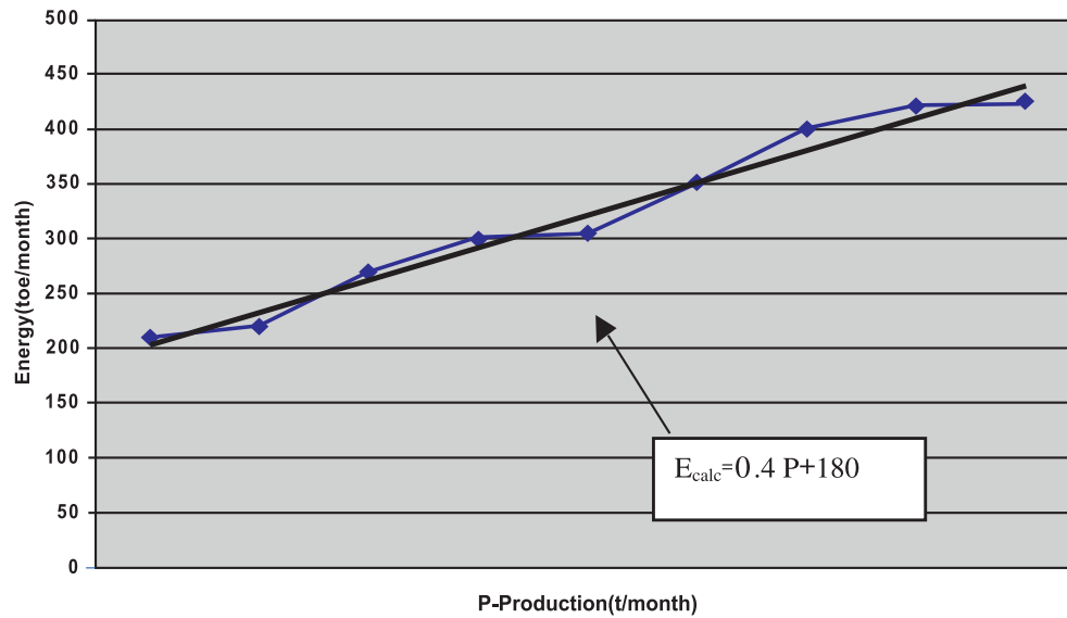
Figure 9.11 Energy-Production Relationships for Foundry
