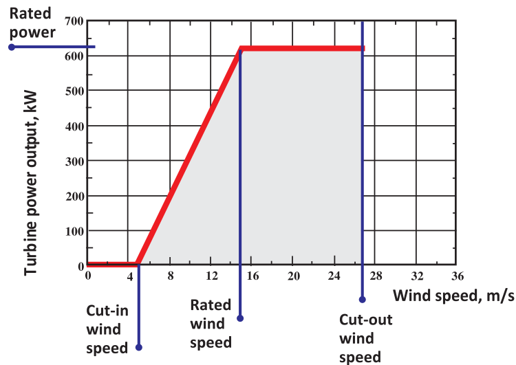
Figure 11.14 Idealised Power Curve for a Wind Turbine
