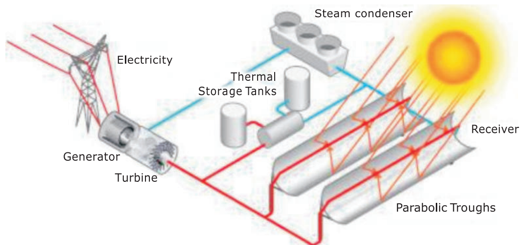
Figure 11.6 Parabolic Trough Collector
