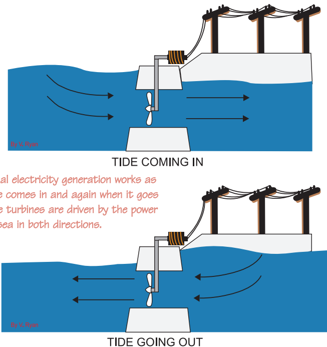
Figure 11.24 Tidal Energy
