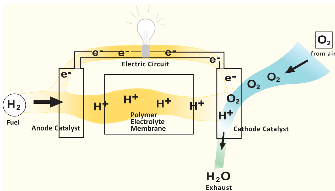
Figure 11.20 Fuel Cell
