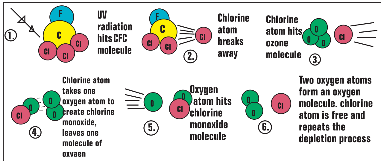
Figure 10.5 Chemistry of Ozone Depletion Process
