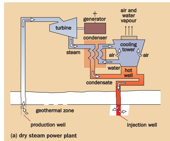
Figure 11.26 Dry Steam Power Plant
