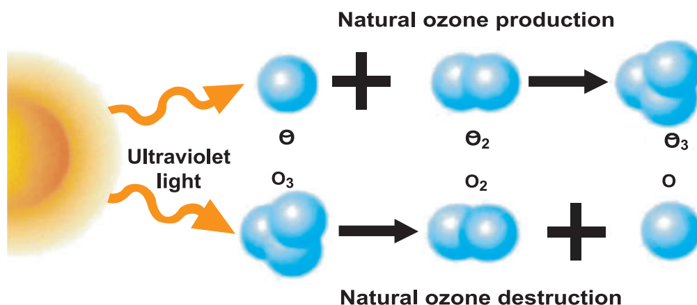
Figure 10.4 Ozone Formation and Destruction
