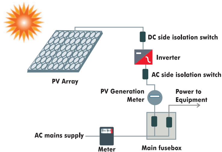
Figure 11.9 Grid Connected Solar
