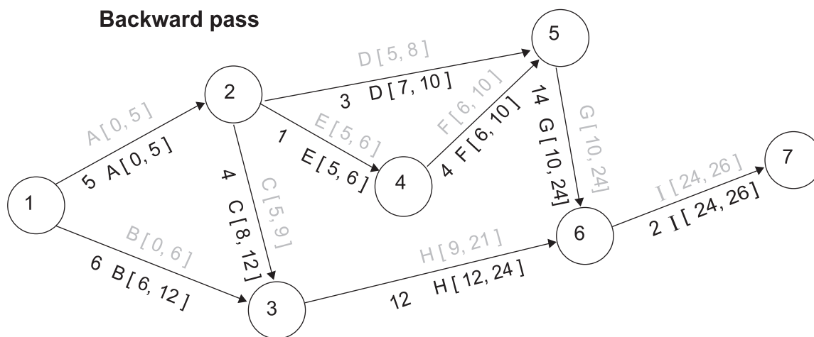
Figure 8.6 Network with LS and LF time in Backward Pass
