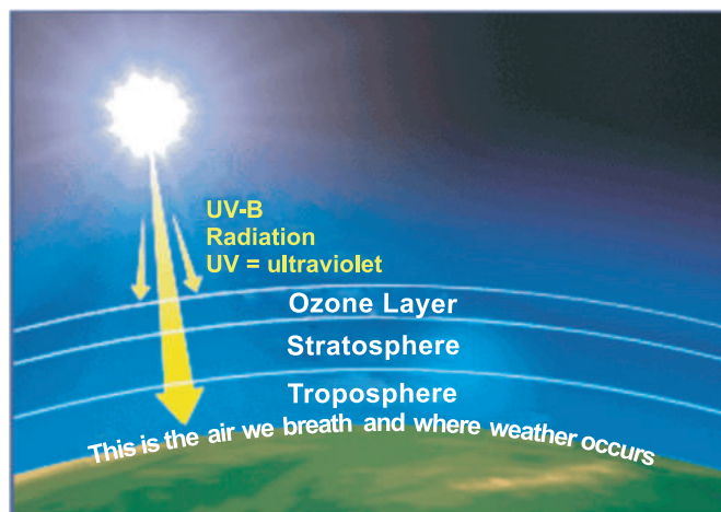
Figure 10.3 Ozone Layer
