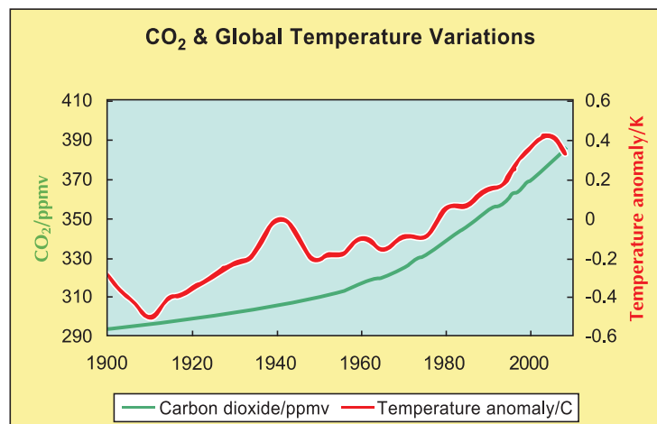
Figure 10.7 Rising Global Temperatures
