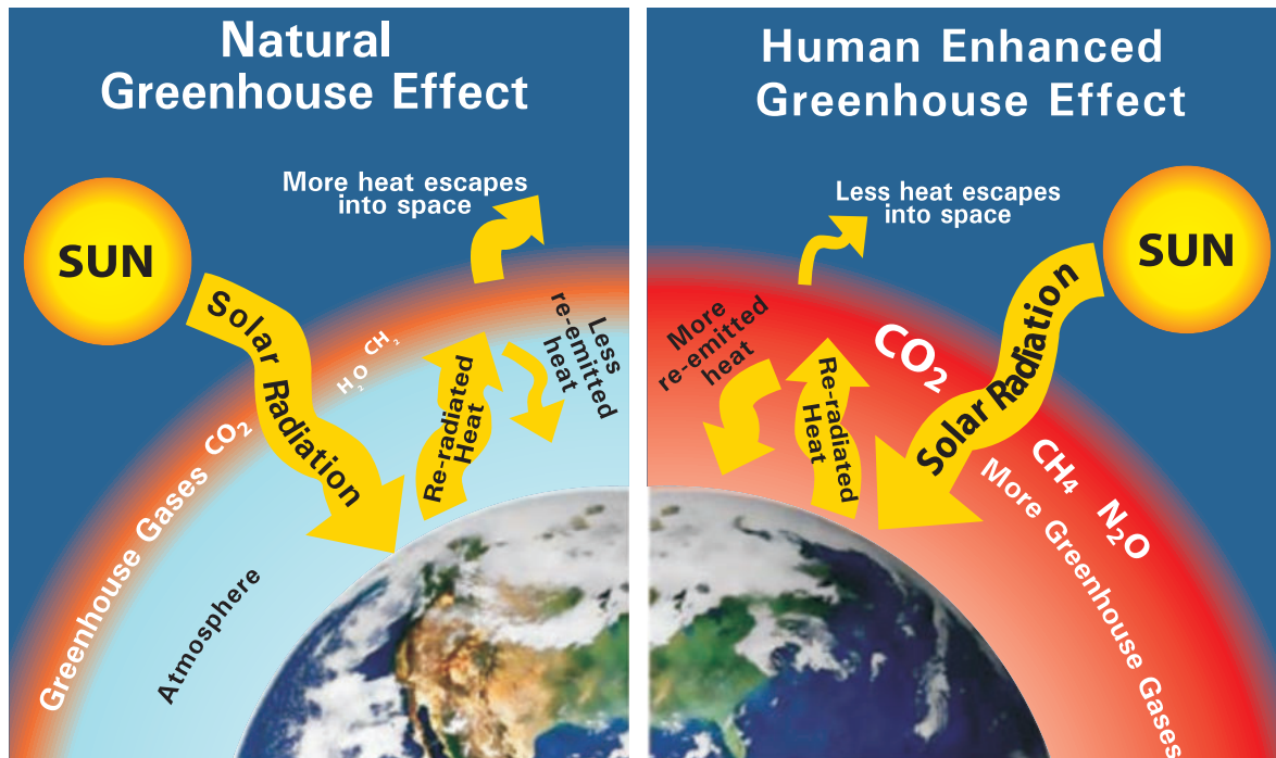
Figure 10.6 Greenhouse Effect
