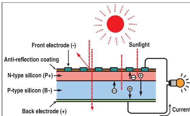
Figure 11.7 Solar Photovoltaic Effect
