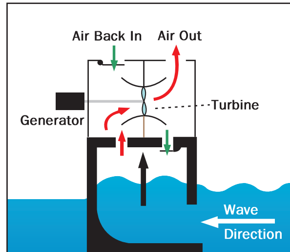
Figure 11.23 Wave Energy
