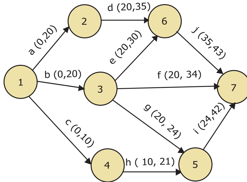
Figure 8.7 ES and EF for Network in Forward Pass
