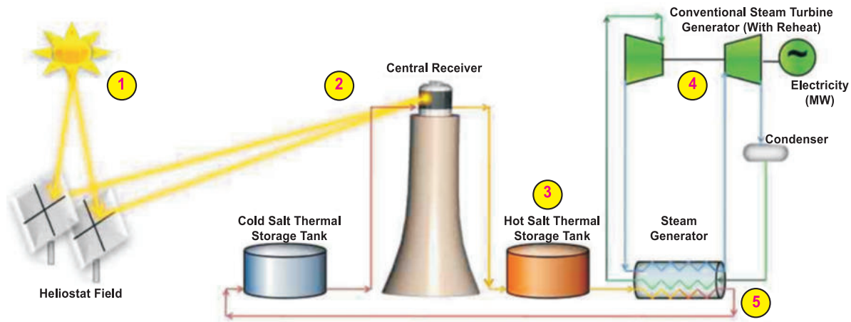
Figure 11.5 Solar Thermal Power Stations
