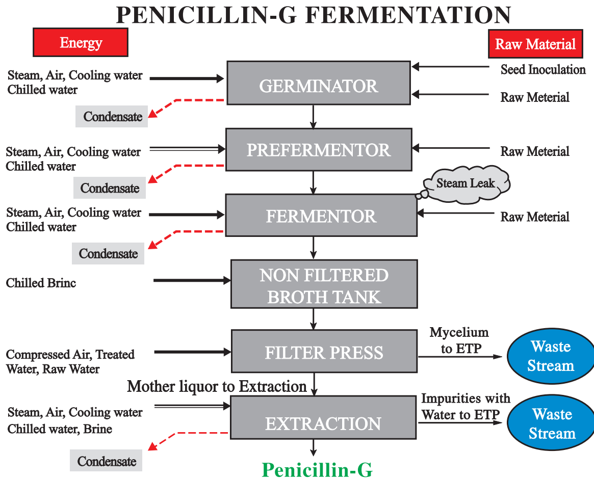
Figure 4.1 Flow Chart for Penicillin-G Manufacture
