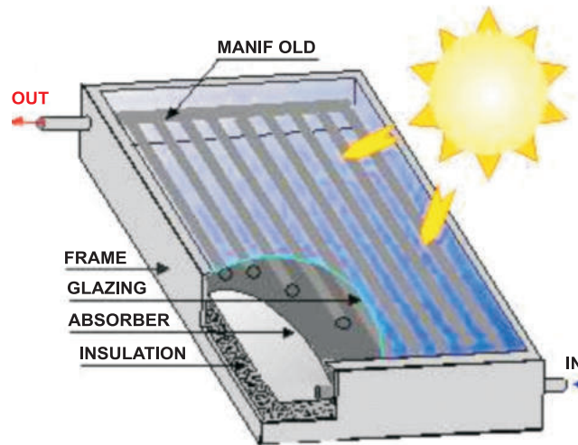
Figure 11.2 Solar Flat Plate Collector
