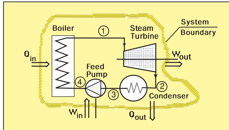
Figure 5.6 Energy Balance in Power Plant Cycle
