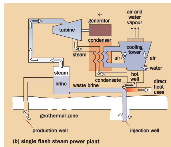
Figure 11.27 Flash Steam Power Plant
