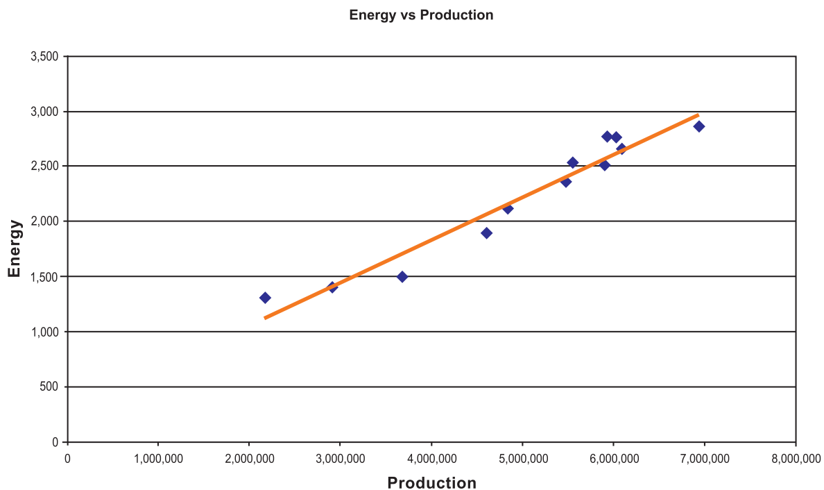
Figure 9.10 XY Chart for Energy-Production Relationship
