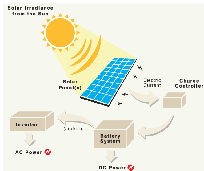
Figure 11.8 PV System
