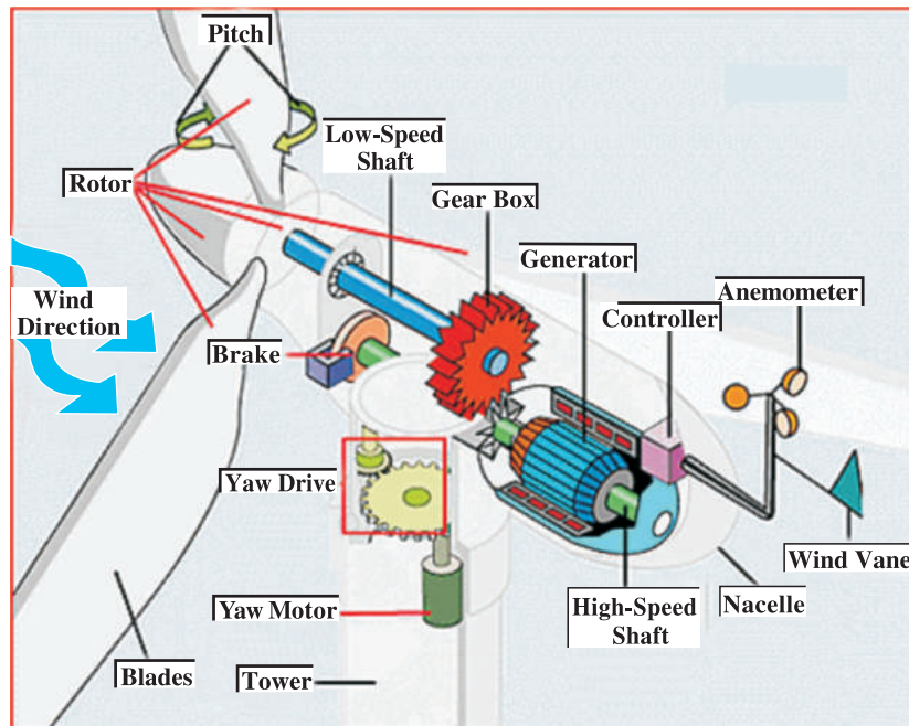
Figure 11.13 Nacelle Assembly
