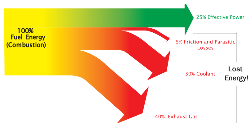
Figure 5.9 Sankey Diagram for an Internal Combustion Engine
