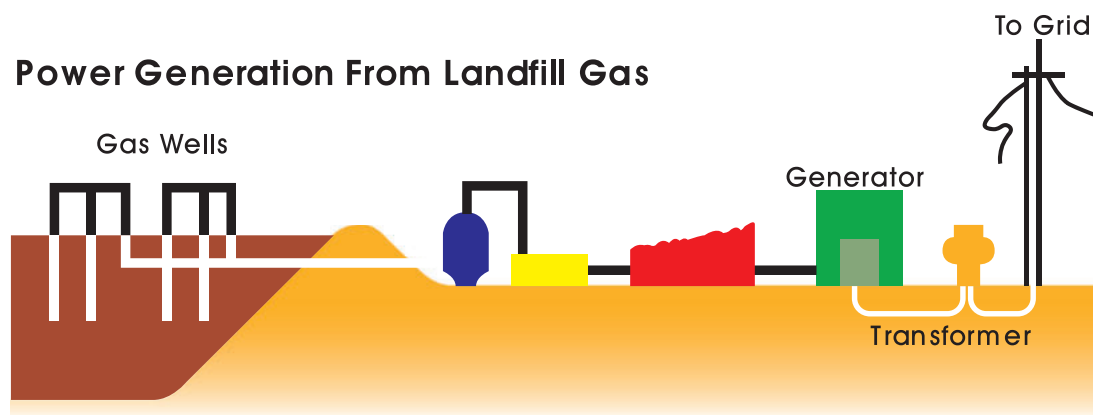
Figure 11.21 Energy from Wastes
