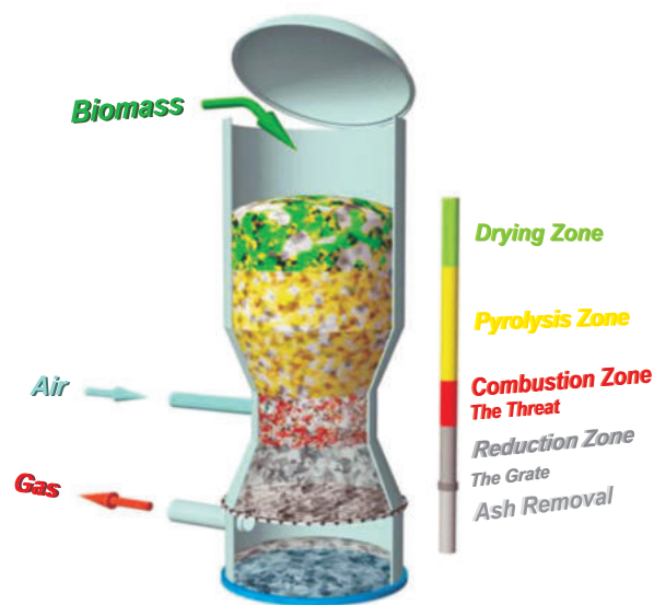
Figure 11.16 Gasifier
