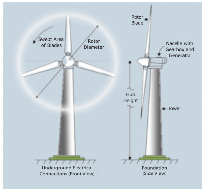
Figure 11.12 Rotor and Blades
