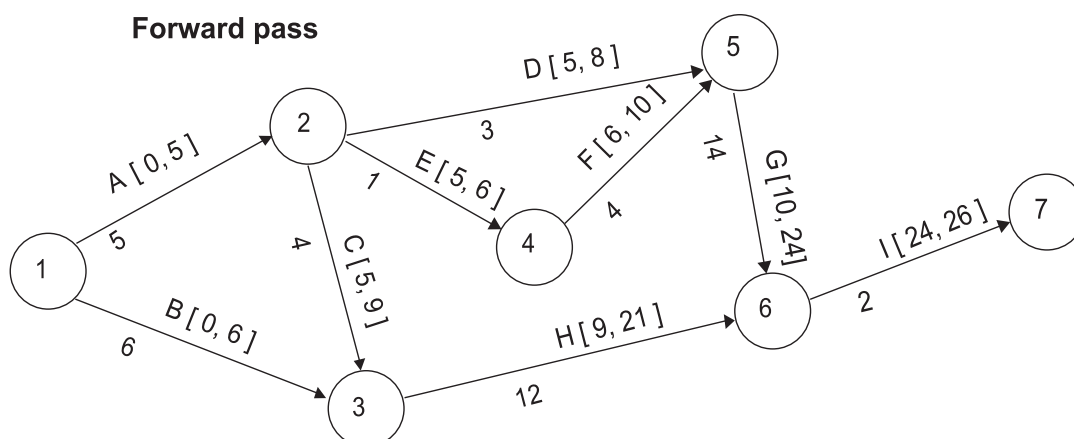
Figure 8.5 Network with ES and EF time in Forward Pass
