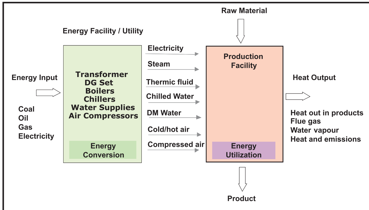
Figure 5.8 Plant Energy Systems
