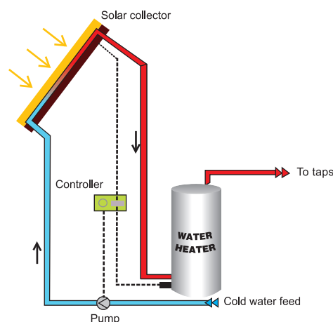
Figure 11.1 Solar Water Heating System
