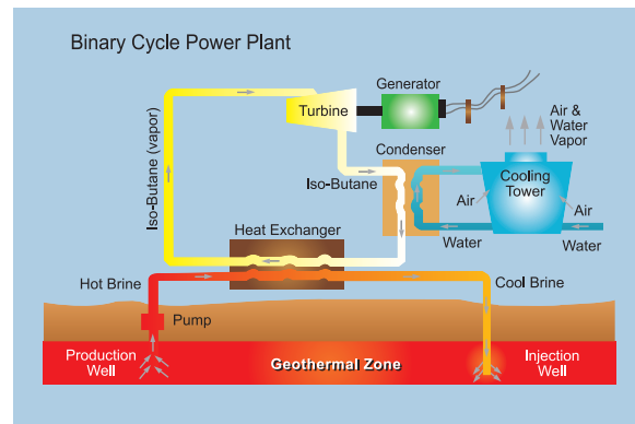
Figure 11.28 Binary Cycle Power Plant
