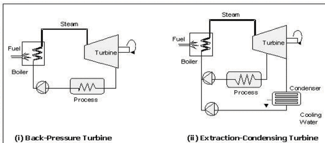
Schematic diagrams of steam turbine cogeneration systems
